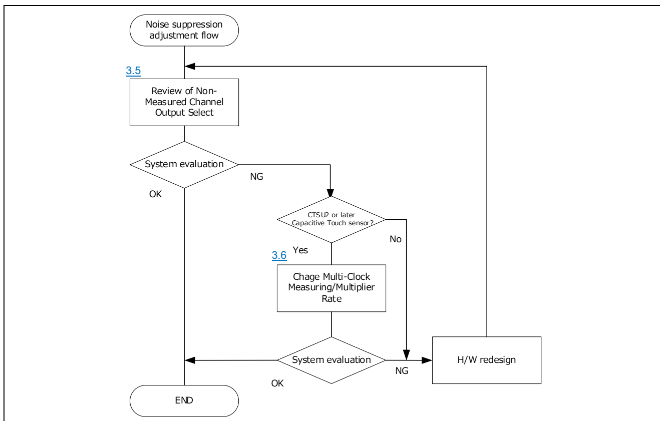
Figure 2-2 Noise suppression adjustment flow
