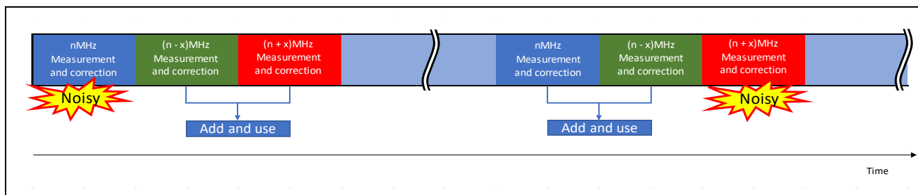
Figure 3-16 Image of multi-clock measurement (3-frequency measurement)
