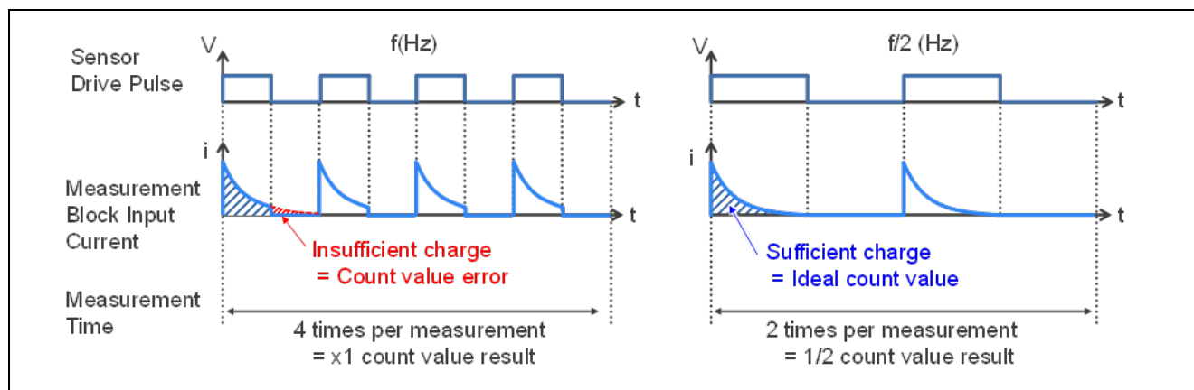
Figure 3-10 Image of CTSU measurement
