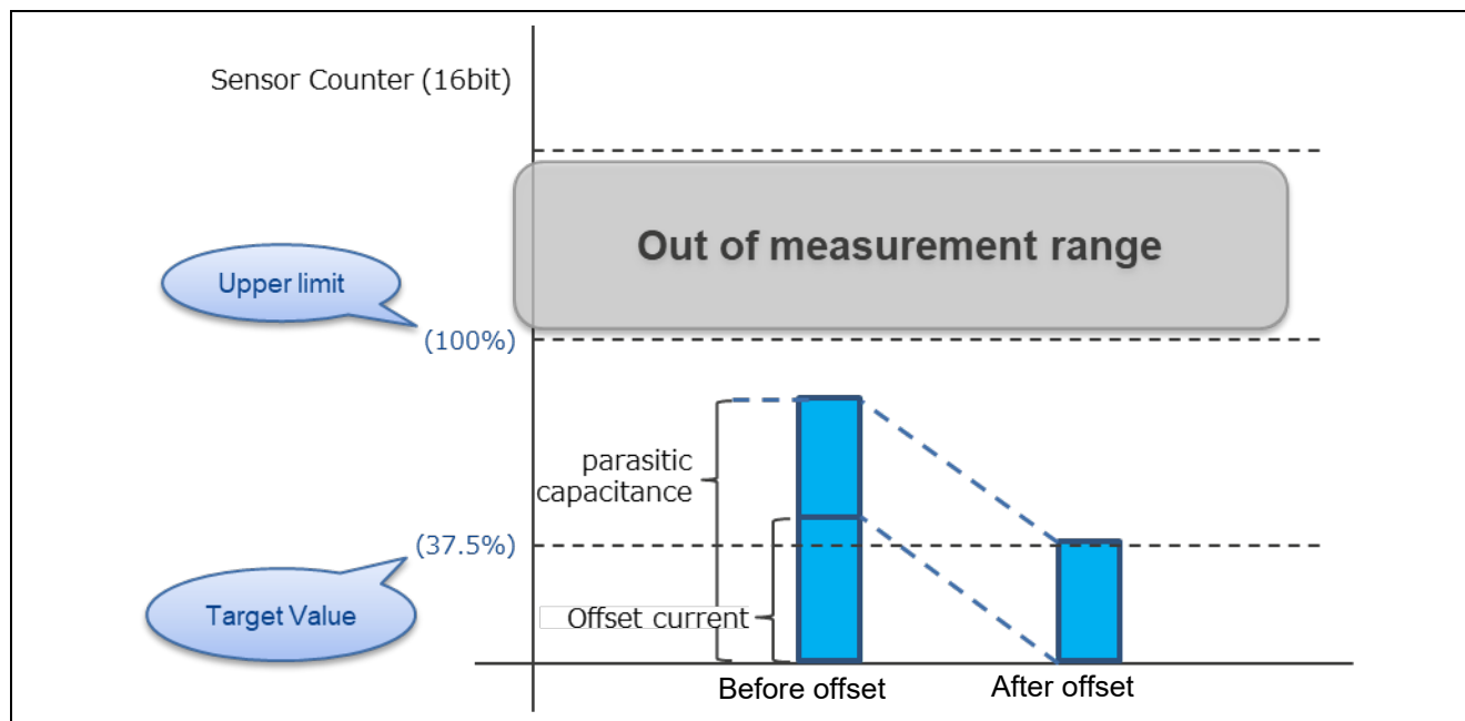
Figure 3-4 Offset Tuning Process of Self-Capacitance Method
