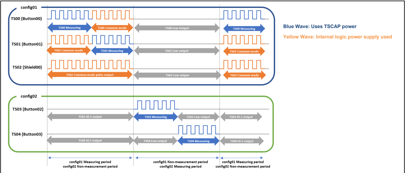
Figure 3-14 Image of TS terminal measurement
