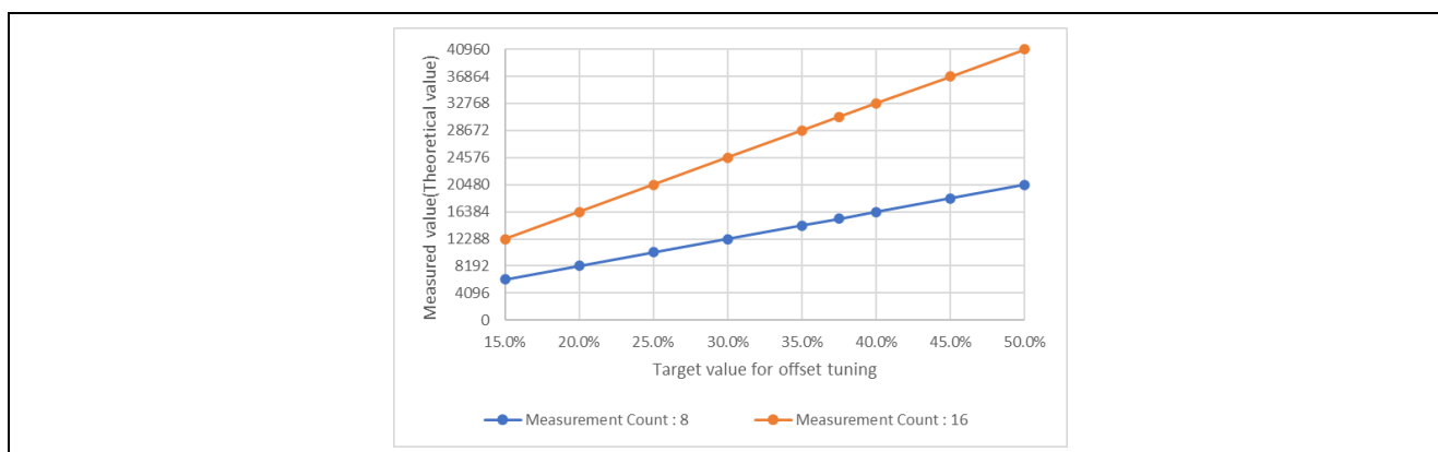
Figure 3-6 Measurement value (theoretical value) with respect to "Target value of Offset Tuning" when the number of measurements is changed
