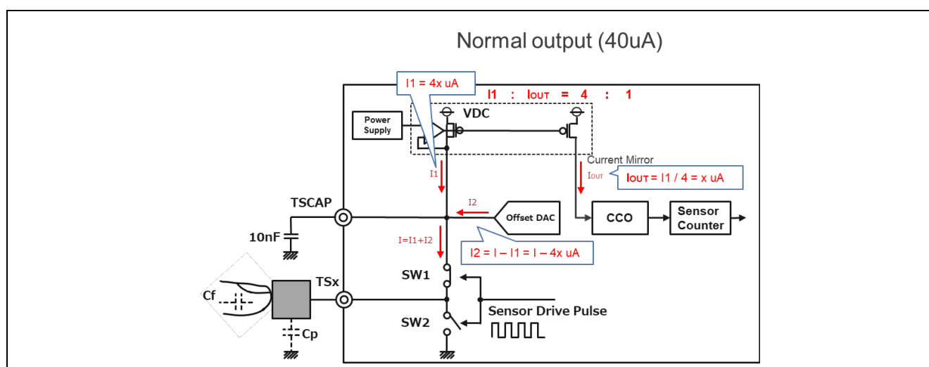
Figure 3-11 Measurement image when normal current (40uA) is used
