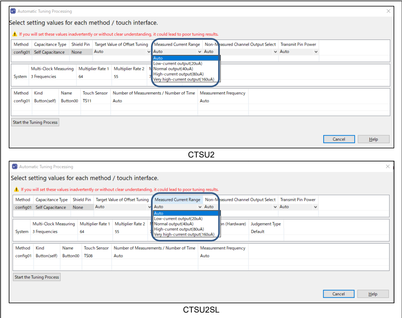
Figure 3-12 Setting of "Measured Current Range"
