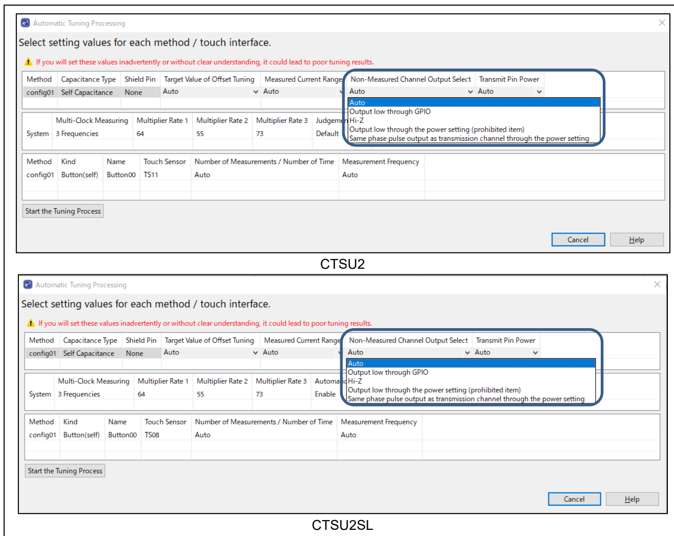
Figure 3-15 Setting of "Non-Measured Channel Output Select"
