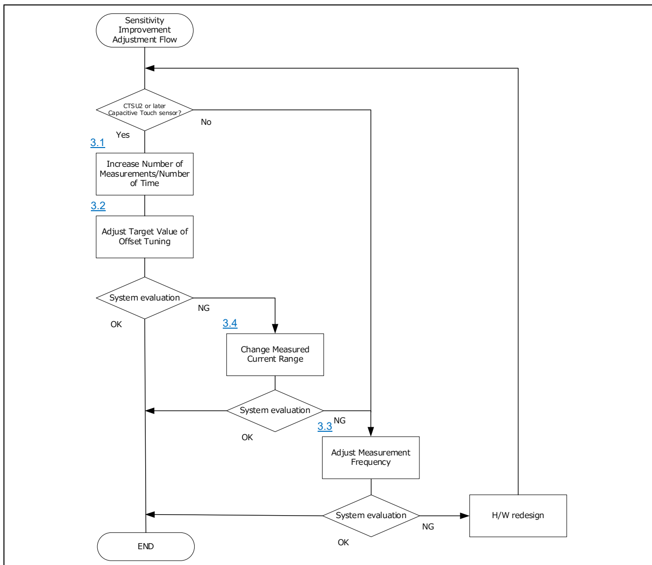
Figure 2-1 Sensitivity improvement adjustment flow
